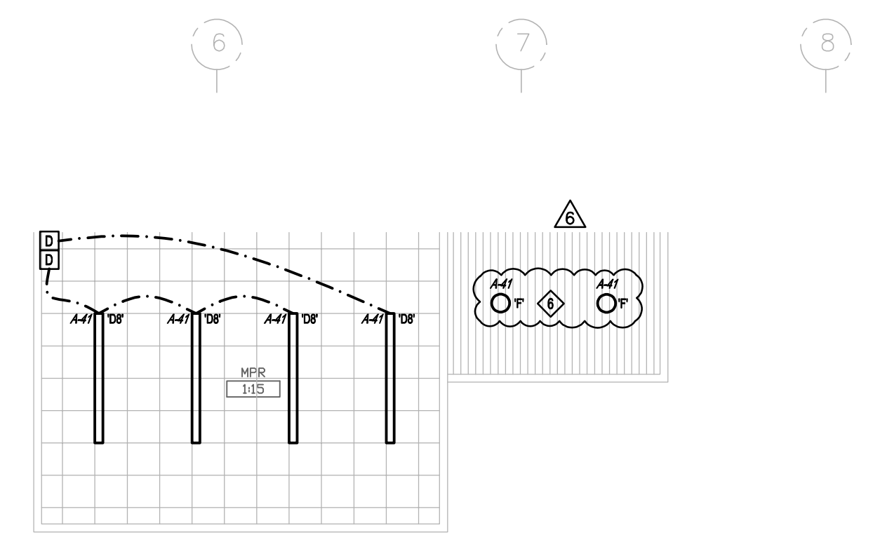
2 MPR / SAUNA FLOOR PLAN LIGHTING EL2.1 SCALE: 1:100
