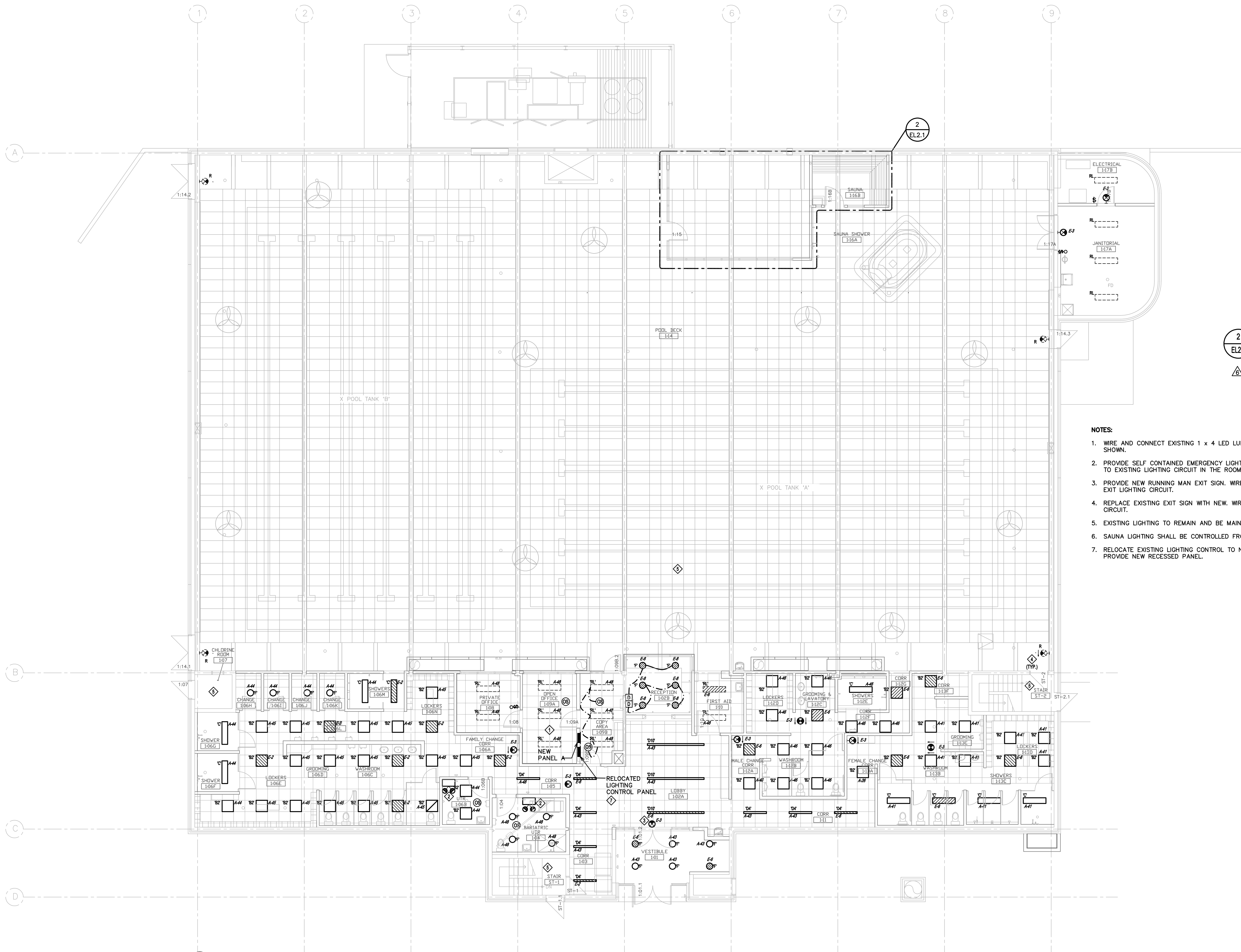
1 MAIN FLOOR PLAN LIGHTING EL2.1 SCALE: 1:100
